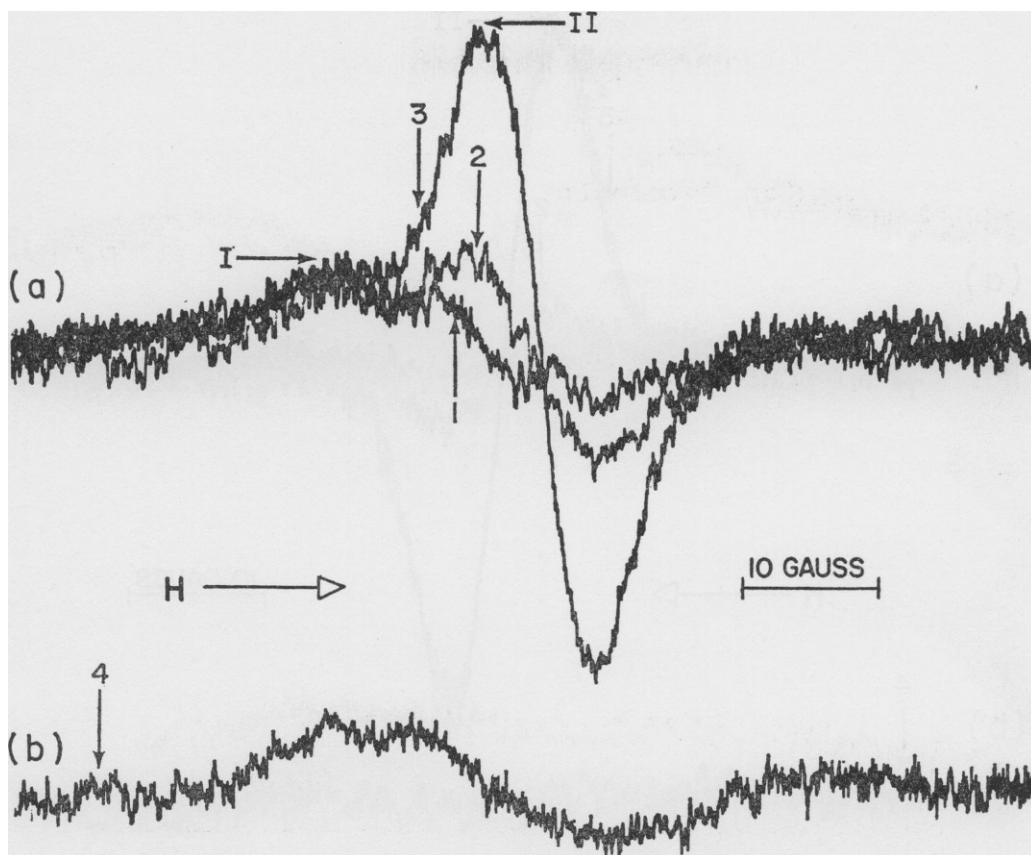
FIGURE 4 ESR spectra of ac-21 . (a): 1, Magnetic field scan in absence of light; 2, Magnetic field scan with 540\text{ m}\mu light; 3, Magnetic field scan with red light. (b): 4, Retrace of magnetic field scan in the dark after light experiments.
