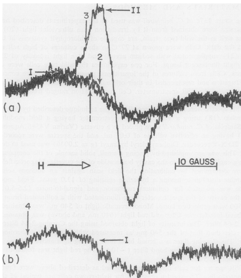
FIGURE 1 ESR spectra of wild type C. reinhardtii . (a): 1, Magnetic field scan in the absence of illumination; 2, Magnetic field scan with 540 m\mu light; 3, Magnetic field scan with red light (Corning 2-64 filter); I, Multicomponent resonance at g = 2.0036 ; II, Narrow resonance, line width = 8.2 gauss and g = 2.0023 . (b): 4, Retrace of magnetic field scan in the dark after light experiment. Only signal I remains.
